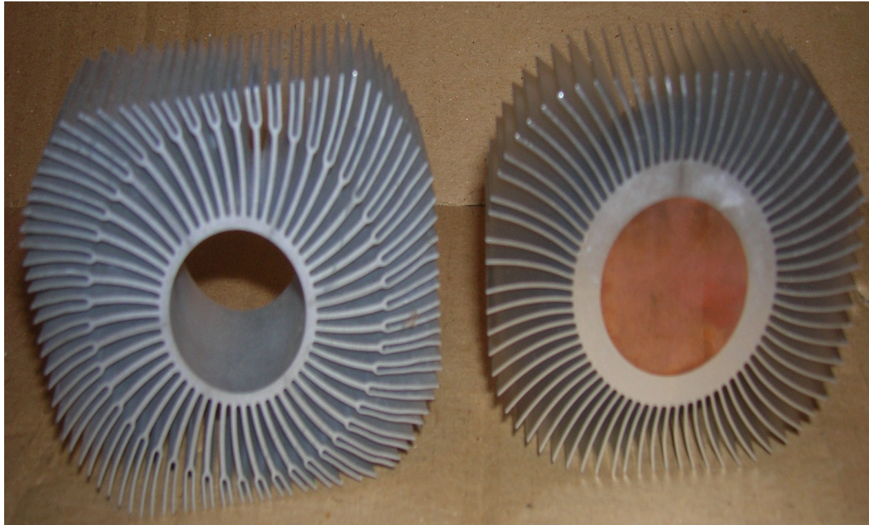
Precision Copper inserted into the Aluminium Heatsink to enhance Thermal Conductivity
